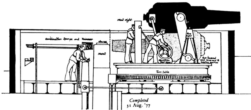
Longitudinal section of the Temeraire's barbettes with the gun raised for firing in the fore-and-aft line, or (in lighter shade) lowered for loading.
