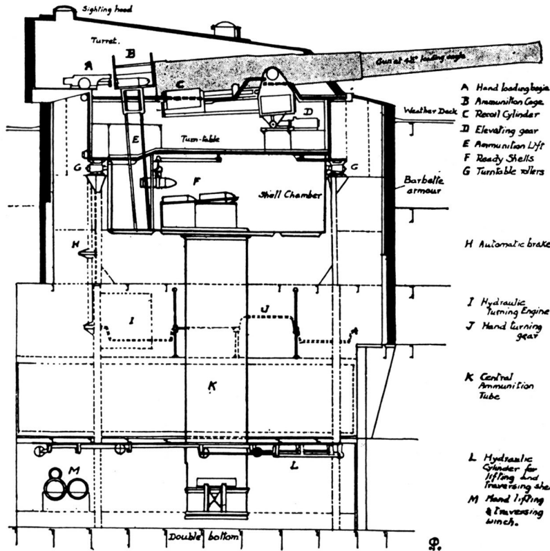
Section of Formidable's barbette showing the ammunition hoist interrupted at the shell chamber instead of being continuous from magazine to guns as in previous classes.
